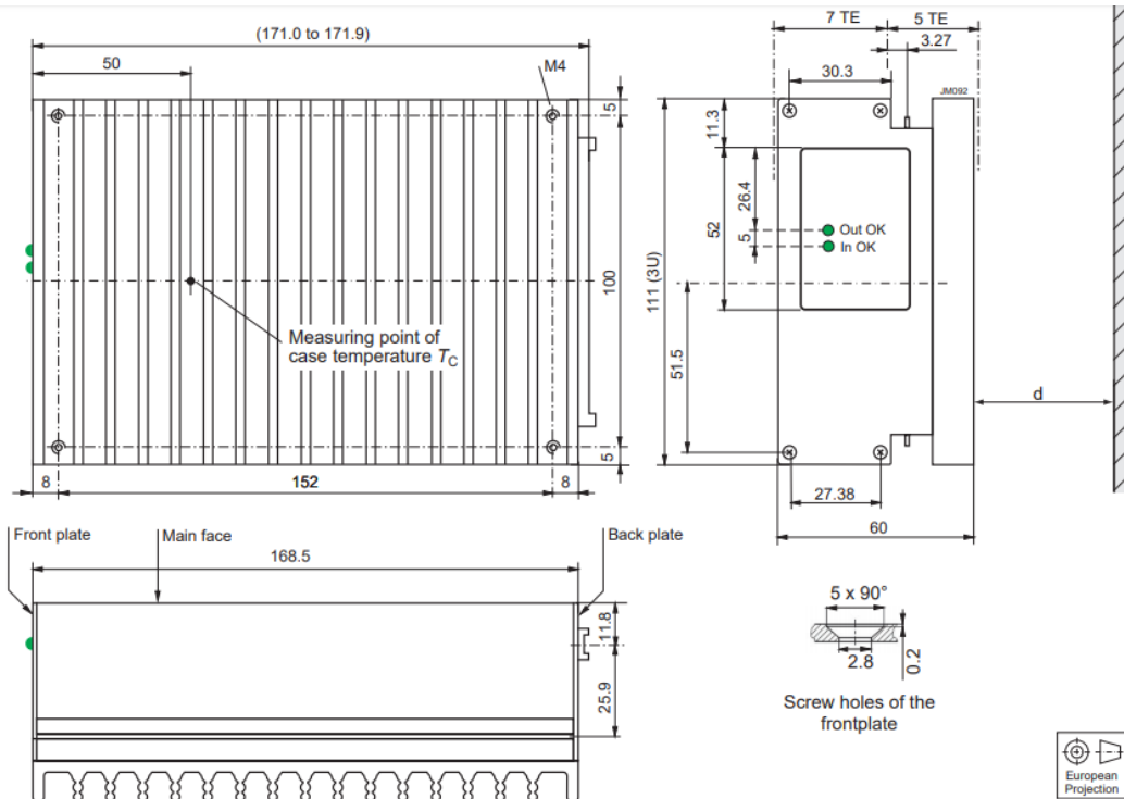
Figure 2. LR models dimension. d > 15\text{mm} .
