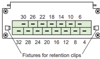
Figure 1. Connector Pin description
