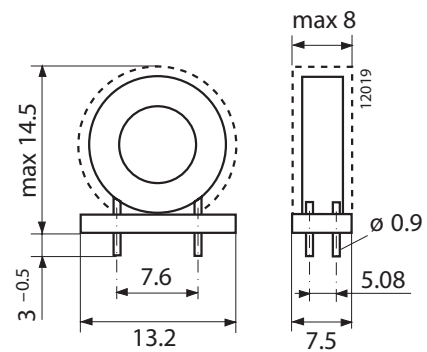
Fig. 11 Common mode choke LP 183, weight 7 g
