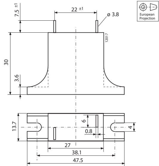
Fig. 9 Differential mode choke L 20-7, weight 30 g
