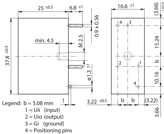
Fig. 8 Filter blocks FP weight 30 g
