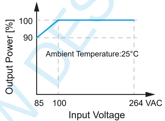
Figure 2. Input Voltage Derating Curve
