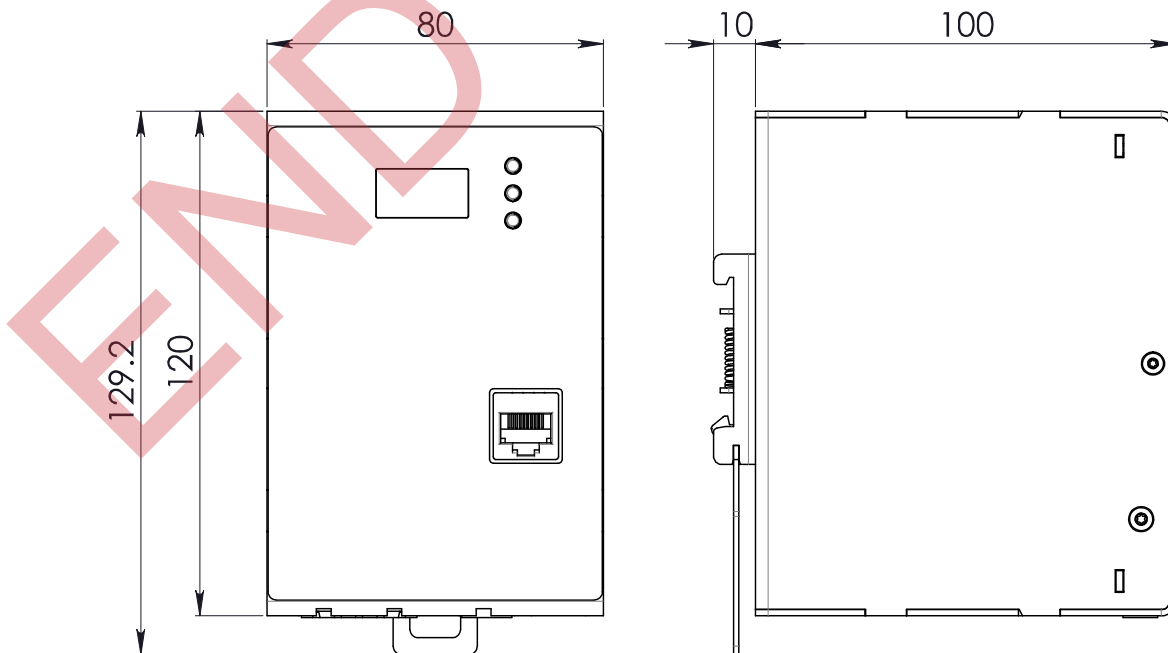
Figure 2. Mechanical Drawing
