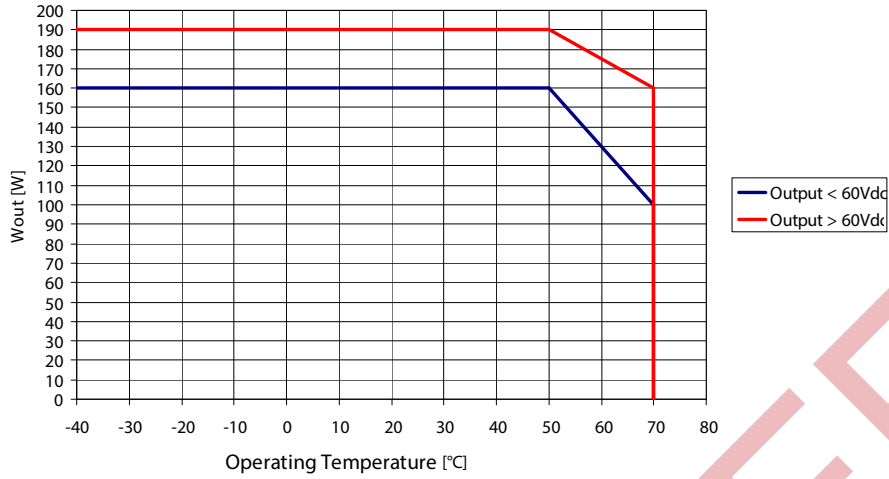
Figure 1. Derating curve
